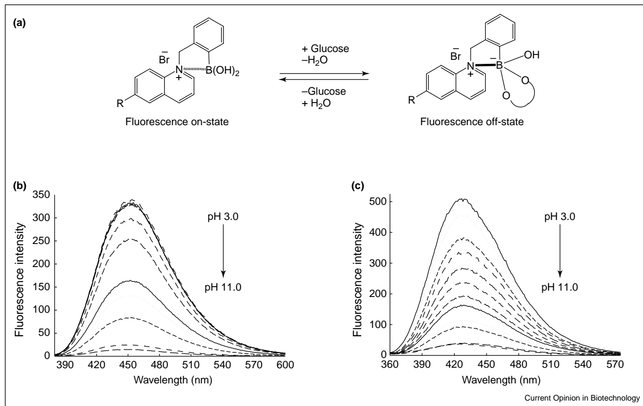
Signaling mechanism. (a) Schematic representation of the charge neutralization-stabilization mechanism with regard to glucose sensing. The bold-line between the N^+ and boron atom in the structure shown on the right-hand side of the equation indicates the increased interaction between them, and is not intended to show covalent bond formation between the two atoms. Emission spectra of (b) o -BMOQBA and (c) o -BMQBA in buffered media. \lambda_{\text{ex}} for BMOQBA and BMQBA was 345 nm and 320 nm, respectively.
