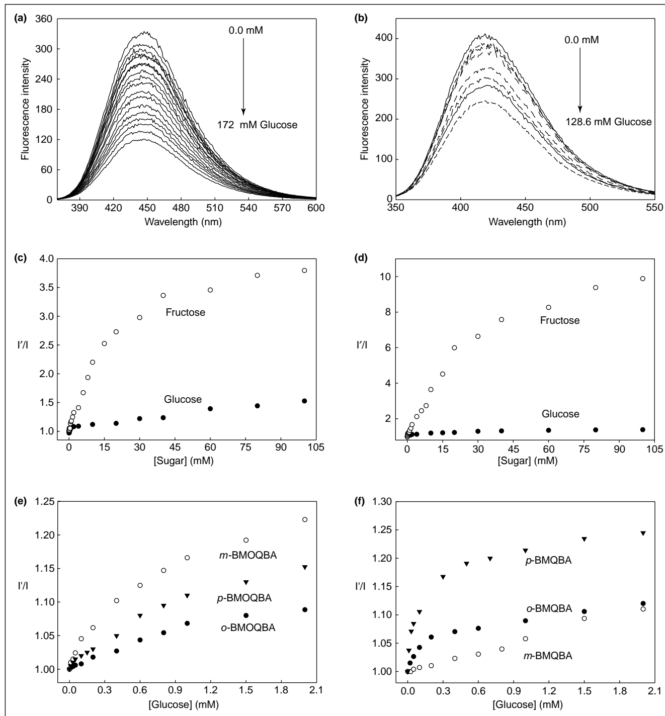
The response of contact lenses to sugars. The emission spectra of (a) an o -BMOQBA- and (b) an o -BMQBA-doped contact lens in the presence of increasing glucose concentrations. \lambda_{ex} was 345 nm for o -BMOQBA and 320 nm for o -BMQBA. The corresponding emission intensity ratio at band maximum for (c) o -BMOQBA- and (d) o -BMQBA-doped contact lenses in the absence ( I' ) and presence ( I ) of both glucose and fructose. The response of different isomers of (e) BMOQBA and (f) BMQBA in the contact lens in the tear glucose concentration range. (Figure adapted from [25**].)
